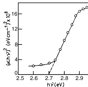
Fig. 2. (\alpha hv)^2 vs hv plot for ZnSe film.
