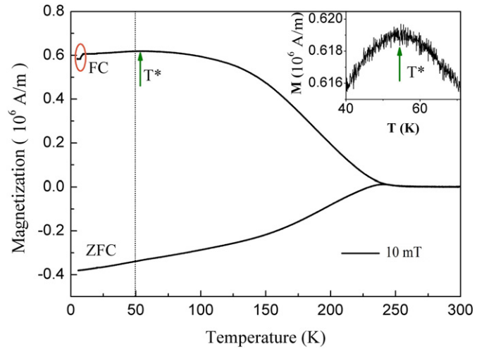
Fig. 2. Temperature dependence of magnetization with ZFC and FC in 10 mT field processes for PSMO/LCMO film. Inset was the enlarged magnetization curves.
