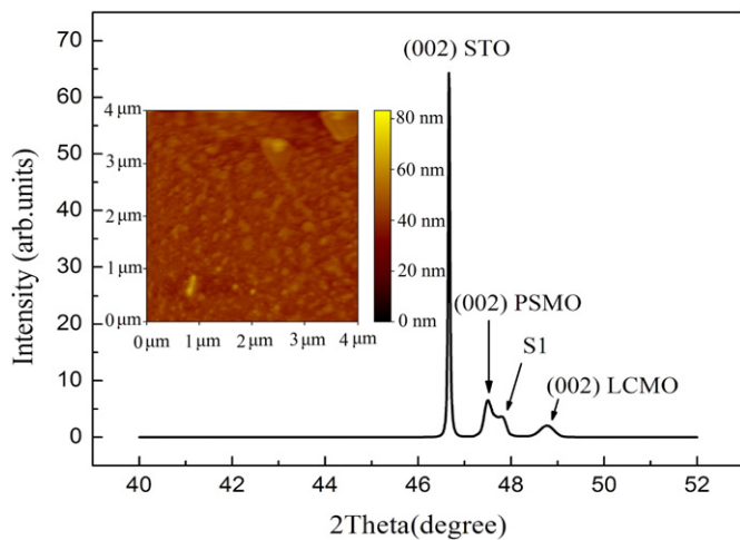
Fig. 1. HRXRD \theta - 2\theta scan centered on the STO (002) peak for PSMO/LCMO bilayer film on (001) STO substrate. Inset: atomic force microscopy contact mode image plotted for an area of 4 \times 4 \mu\text{m}^2 of PSMO/LCMO film.
