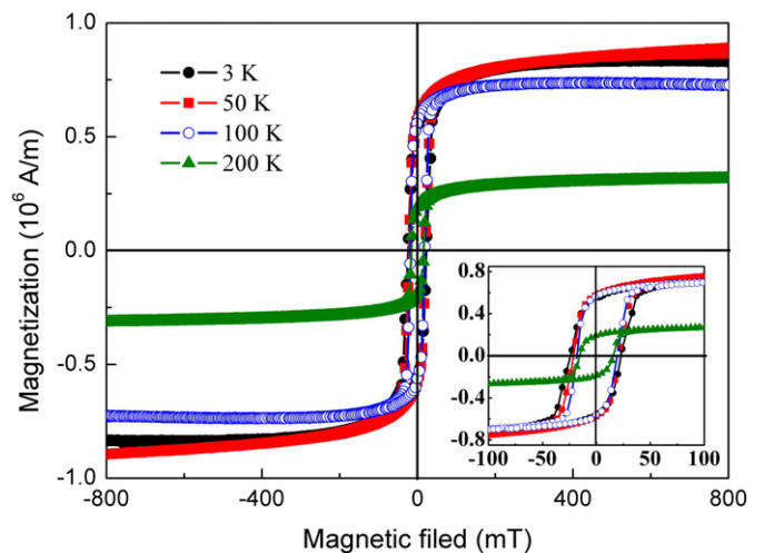
Fig. 3. The FC hysteresis loops of the PSMO/LCMO film at 3 K, 50 K, 100 K and 200 K. Inset shows low field magnetization behavior.
