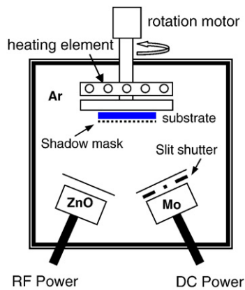
Fig. 1. Schematic of a co-sputter apparatus for fabricating surface textured MZO film.
