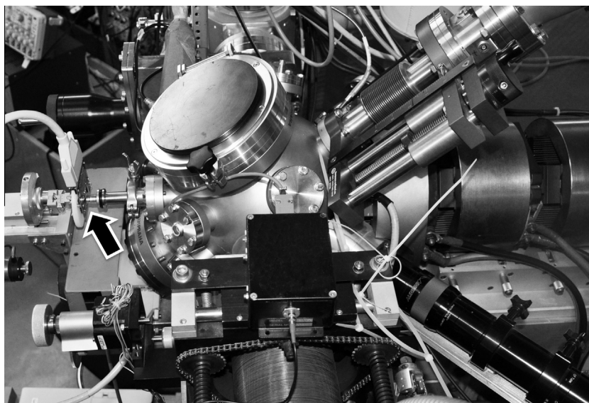
Fig. 1. A side view of the RBI microprobe experimental setup. A quadrupole triplet lens is positioned on the right side of the spherical scattering chamber. Arrow (on left) indicates the position of the in-air microbeam focus with CMS pixel readout chip containing 52 \times 80 pixels mounted for IBIC tests.
