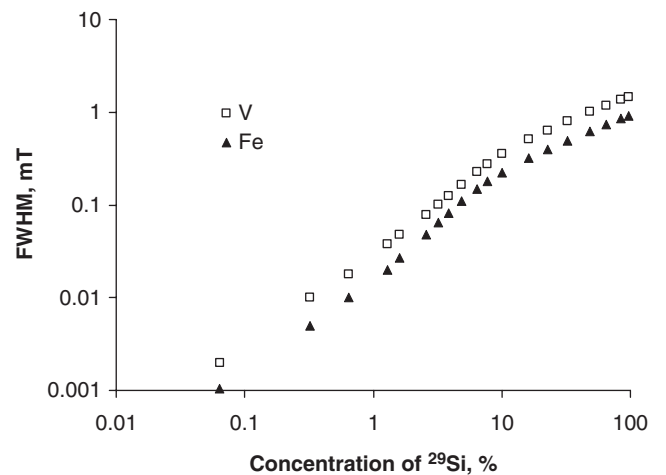
Fig. 1. Dependence of the full-width at half-maximum (FWHM) of EPR lines of V^- and \text{Fe}^+ centers in silicon on magnetic nuclear ^{29}\text{Si} concentration.
