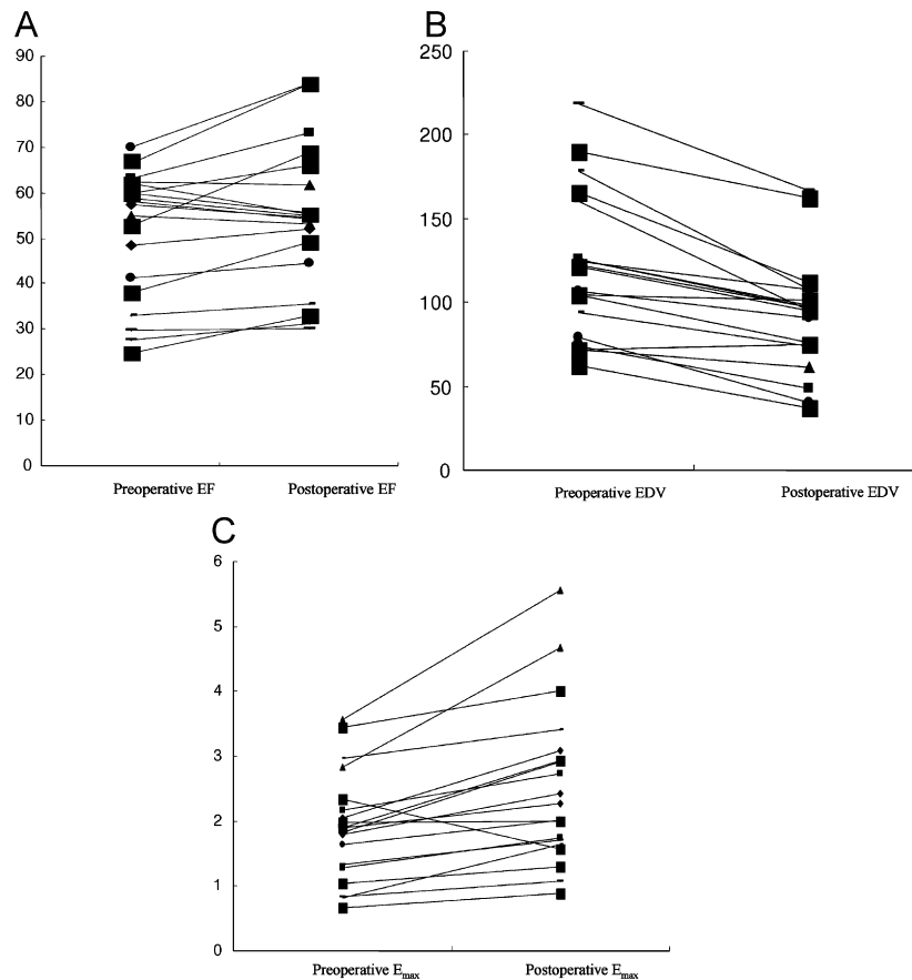
Fig. 1. Postoperative changes of EF(A), EDV(B) and global E_{\text{max}} (C).
