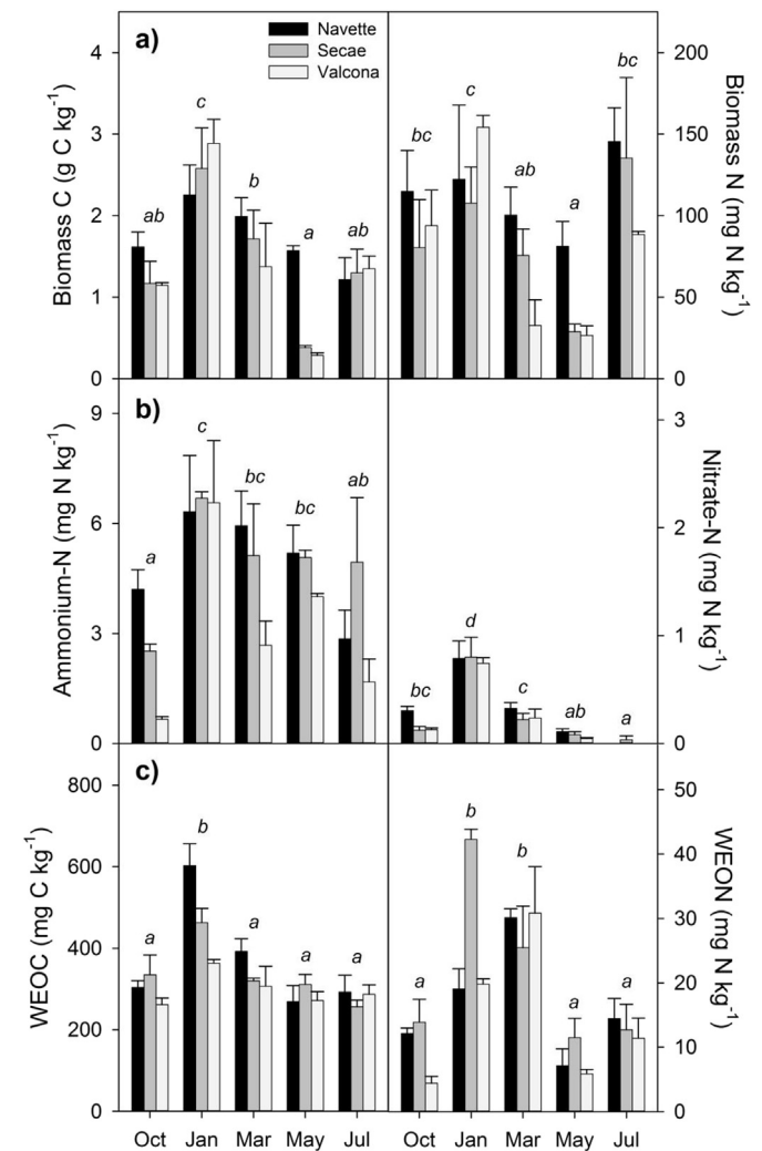
Fig. 2. Seasonal variations in (a) microbial biomass C and N, (b) inorganic N, and (c) water extractable organic C and N. Error bars represent the standard error. Different letters indicate significant differences ( p < 0.05 ) between sampling dates, as determined by the Tukey HSD test.
