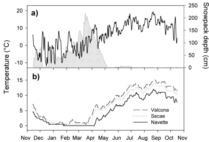
Fig. 1. Variations in (a) daily average air temperatures, snowpack depth (shaded area), and (b) daily average soil temperatures measured at each of the three sites over the experimental period.
