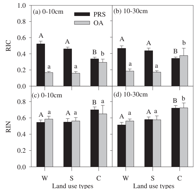
Fig. 2. Annual averages of recalcitrance indexes (RIC and RIN) under different land use. Different capital (PRS) and lowercase (OA) letters over the bars of root indicate statistically significant differences between the land use types. See Fig. 1 for abbreviations.
