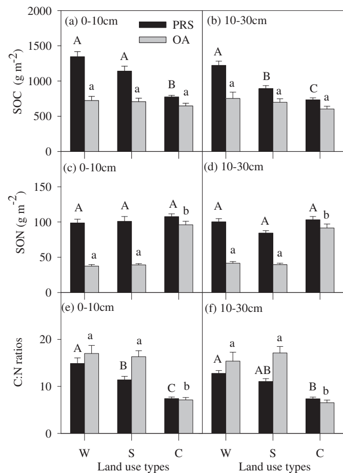
Fig. 1. Annual average of soil organic carbon (SOC), nitrogen (SON) and C:N ratios under different land use. Different capital (plant rhizosphere, PRS) and lowercase (open area, OA) letters over the bars of root indicate statistically significant differences between the land use types. Abbreviations: W, woodland; S, shrubland; C, cropland.
