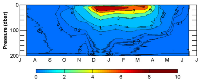
Figure 3. The Seasonal Cycle of Chlorophyll in Marguerite Bay
