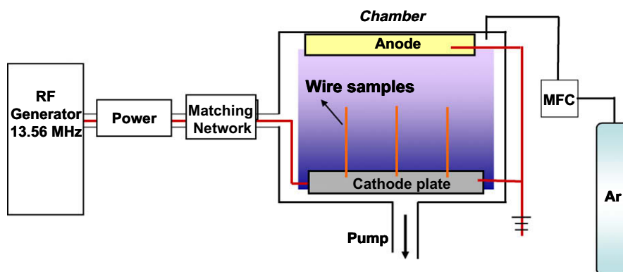
Fig. 1. Schematic shown is an illustration of RF plasma processing of MP35N alloy wires.
