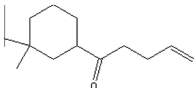
Fig. 1. 1-(3,3-Dimethylcyclohexyl)pent-4-en-1-one.
