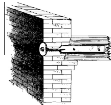
Fig. 1. Image of wall-diaphragm connection (International Library of Technology, 1923 [13]).
