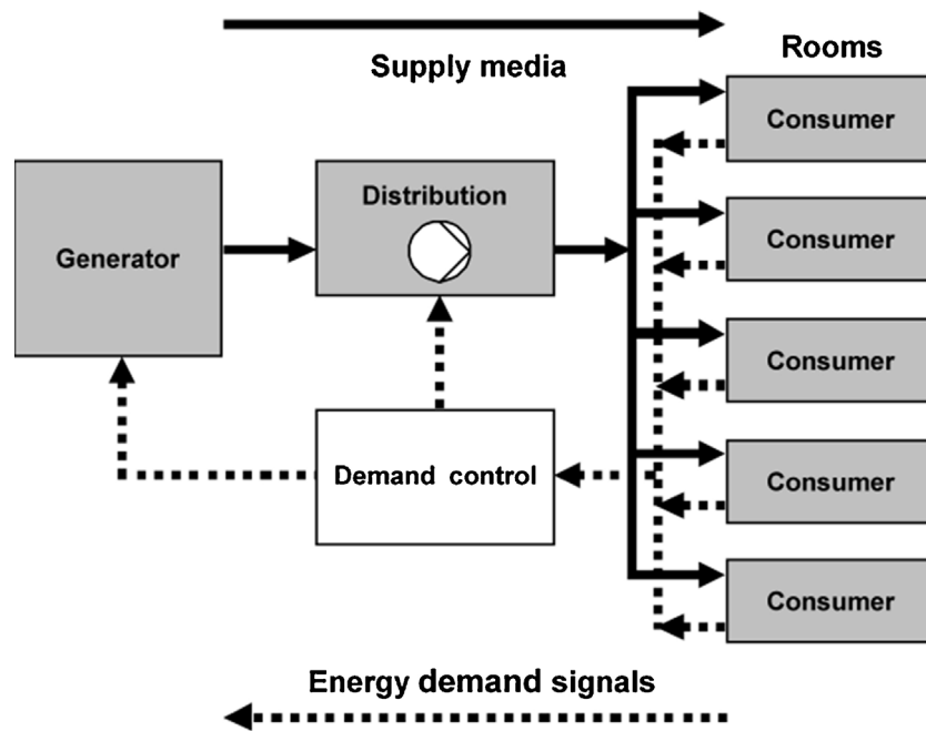
Fig. 1. Demand control according to EN 15232.
