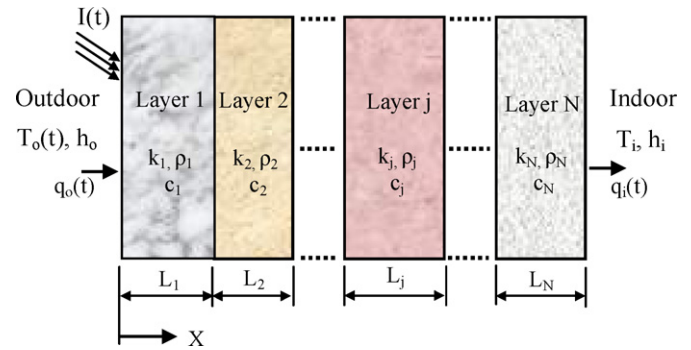
Fig. 1. N-layered composite wall.
