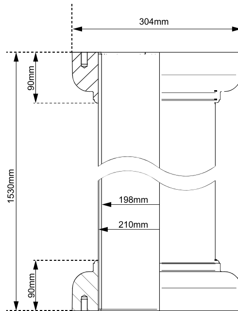
(b) Elevation view of the specimen
