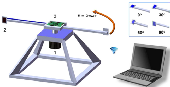
Fig. 1. Schematics of the dynamic tester (1 Motor; 2 Testing platform; 3 Central controlling panel; Inset: Testing platform can be adjusted in different angles).
