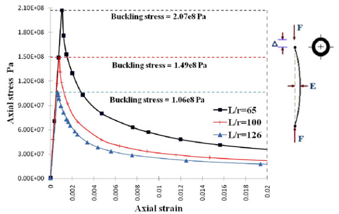
Fig. 2. The axial strain–axial stress responses of the struts with slenderness ratios of L/r = 65, 100 and 126 [7].
