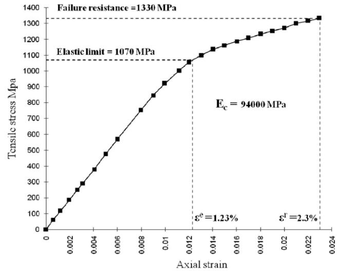
Fig. 1. The strain–stress response of the cables [16].
