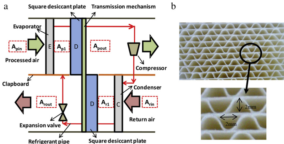
Fig. 1. Operating principle of the dehumidifier using solid desiccant: (a) single-stage dehumidifier; and (b) square desiccant plate material.
