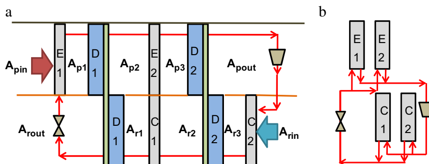
Fig. 2. Operating principle of the multi-stage desiccant dehumidifier: (a) operating principle; and (b) pipeline connection of the heat pump.
