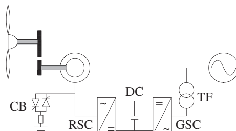
Fig. 3. Doubly-fed induction generator.
