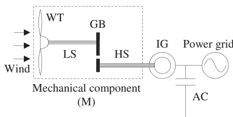
Fig. 1. Constant speed induction generator.
