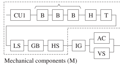
Fig. 2. Reliability model of constant speed IG.
