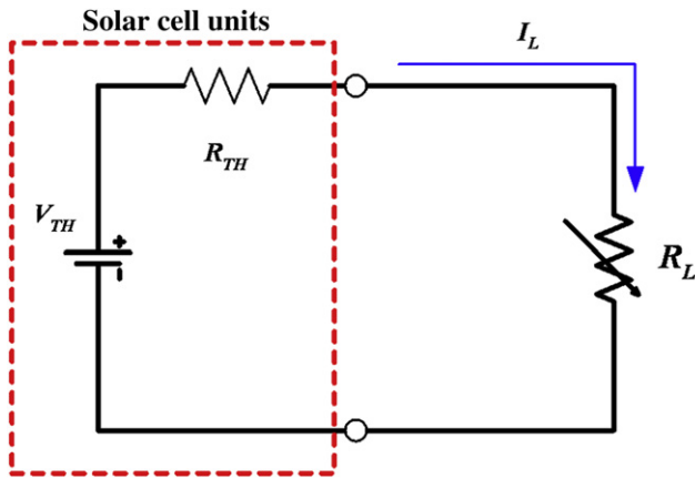
Fig. 1. Schematic demonstration of maximum power transfer for solar cell unit.
