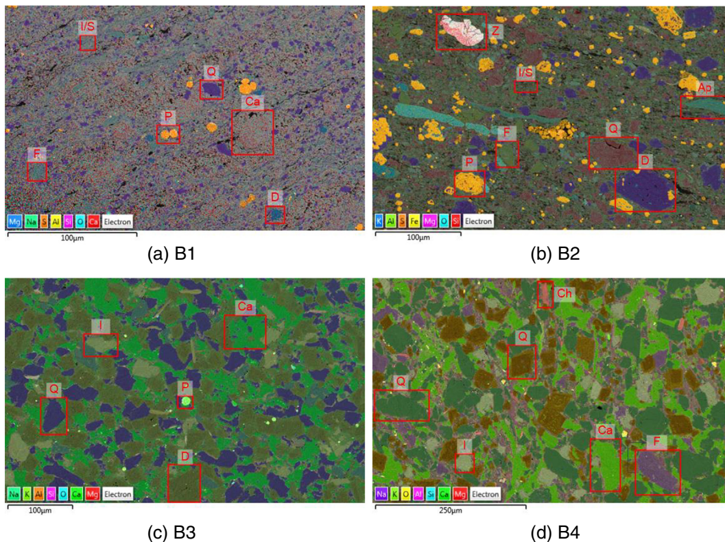
Fig. 2. Elemental maps of rock samples from EDS analysis [10 kV, 3200 nA, and 150 \text{ nm} image resolution] (Q: Quartz, Ca: Calcite, P: Pyrite, D: Dolomite, I/S: Illite/Smectite, F: Feldspar, Ap: Apatite, Z: Zircon, I: Illite, Ch: Chlorite).
