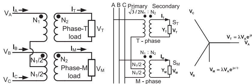
Fig. 2. Scott connection scheme.
