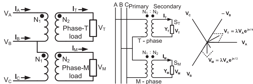
Fig. 1. V–V connection scheme.
