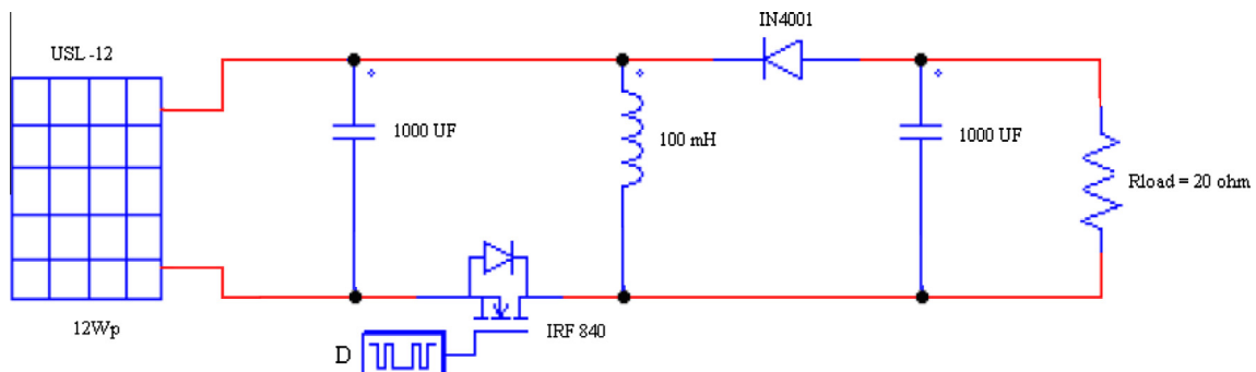
Fig. 2. Schematic of Buck-Boost Converter.
