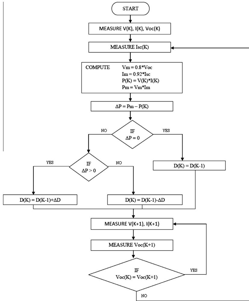
Fig. 1. Flow chart of proposed MPPT algorithm.
