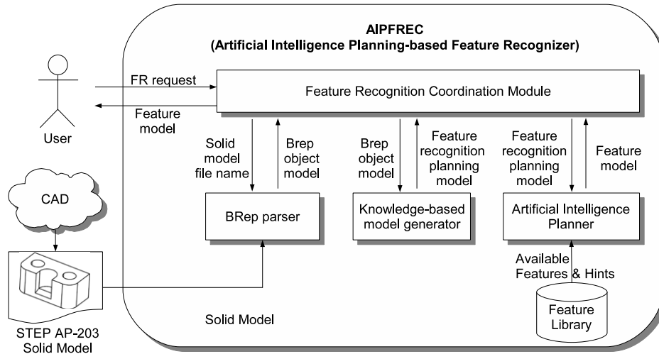
Fig. 3. Proposed feature recognition system architecture.
