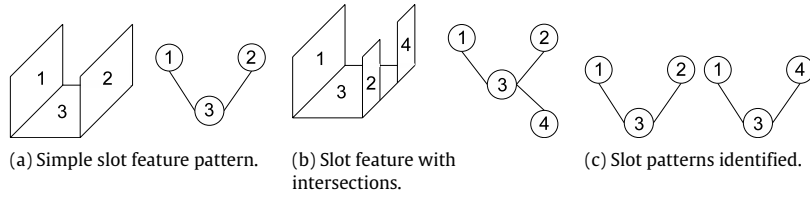
Fig. 1. Limitations of graph-based methods for intersecting features.
