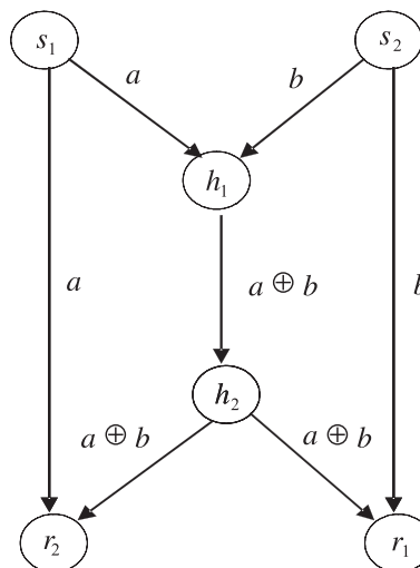
Fig. 1. An example of butterfly network with network coding.
