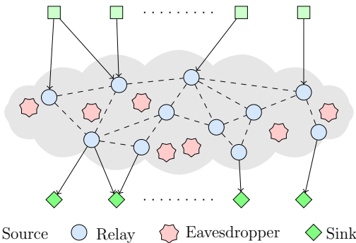
Fig. 1. A general multi-hop network with multiple sources, multiple sinks and multiple eavesdroppers.
