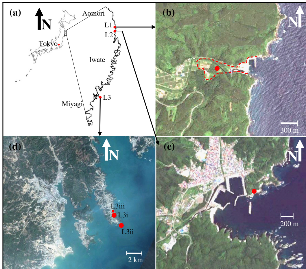
Fig. 1. (a) Boulder sites on the northeast coast of Japan, (b) Settai, Iwate Prefecture ( 39^{\circ} 48' 48''\text{N} , 141^{\circ} 58' 33''\text{E} ), (c) Taro, Iwate Prefecture ( 39^{\circ} 43' 58''\text{N} , 141^{\circ} 58' 47''\text{E} ), and (d) Karakuwa Peninsula, Miyagi Prefecture ( 38^{\circ} 52' 34''\text{N} , 141^{\circ} 39' 31''\text{E} ). Note that circles indicate the location of the boulder site. Fig. 1b–d shows sites before the 2011 tsunami. Source of Fig. 1b–d: Google Earth.
