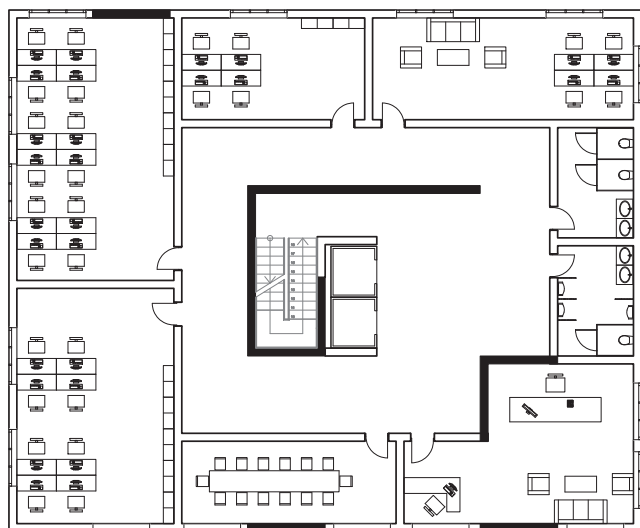
Fig. 1. Example of a desired final layout result. The solid lines represent locations chosen for the shear walls.
