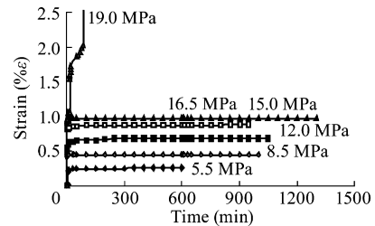
Fig. 3. Creep curves of coal filled with 0 MPa gas.
