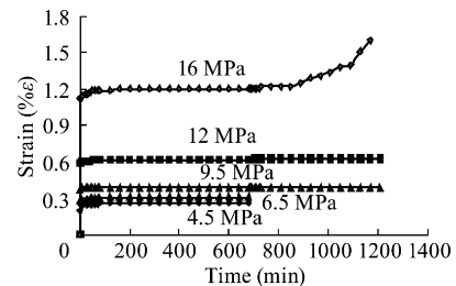
Fig. 4. Creep curves of coal filled with 0.5 MPa gas.
