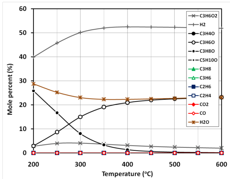
Hydrogenation
