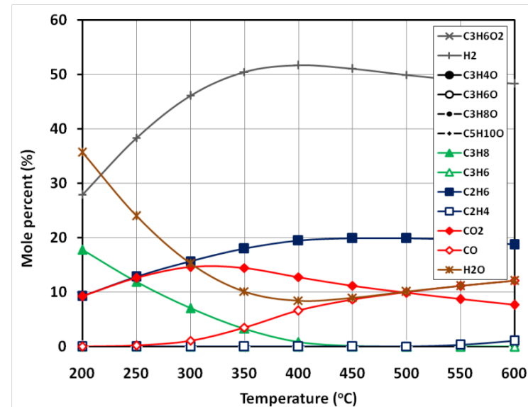
De-oxygenation
