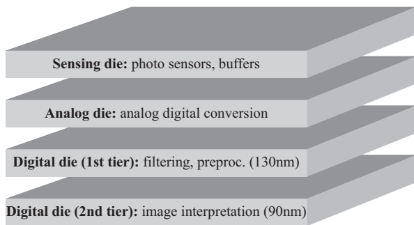
Fig. 1. 3D-VSoC design [16].
