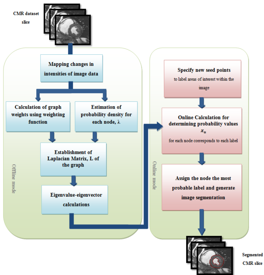
Fig. 1: The proposed random walk technique framework
