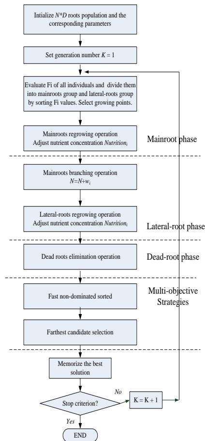
Fig.1 The flowchart of MORSGO algorithm
