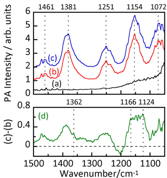
Fig. 2. PA spectra of (a) TiO 2 powder in an oxygen atmosphere, (b) gaseous 2-propanol and (c) TiO 2 powder in an oxygen atmosphere containing 2-propanol, and (d) difference spectra of (c)-(b).
