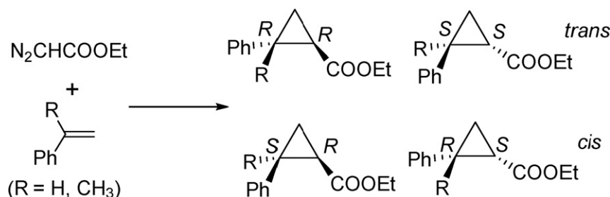
Scheme 1. Cyclopropanation of styrene and \alpha -methylstyrene with ethyl diazoacetate.
