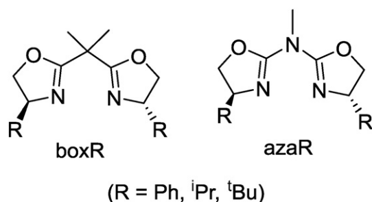
Fig. 1. Ligands used in this work.
