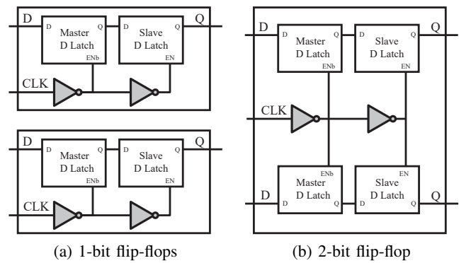
Fig. 1. Internal structure of 1-bit master-slave based flip-flops and 2-bit flip-flop in which the pairs of master-slave latches share the clock driving logic.
