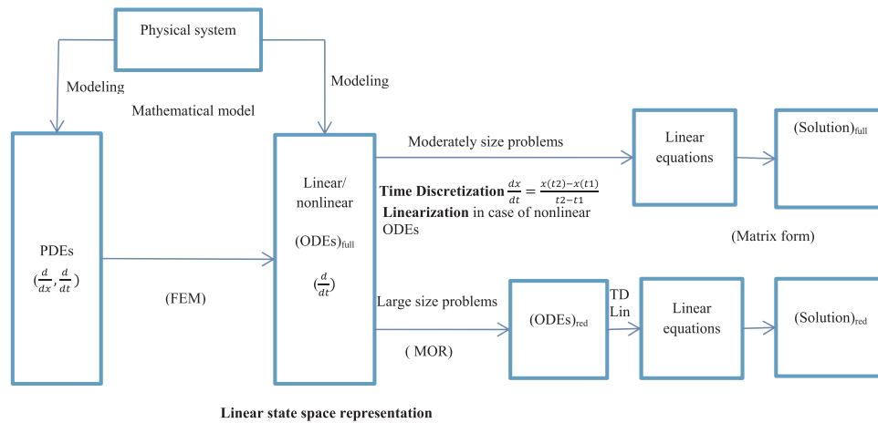
Fig. 1. Typical development flow for complex systems: the big picture, MOR is needed for large size problems, given an ODE of order n , find another ODE of order r , where r \ll n with “essentially” the same “properties” and stability, passivity are preserved. We replace the set of ODEs by a smaller set of ODEs without sacrificing the accuracy of the system behavior.
