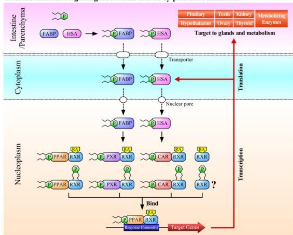
Plausible molecular signaling mechanism elicited by phthalates in humans
