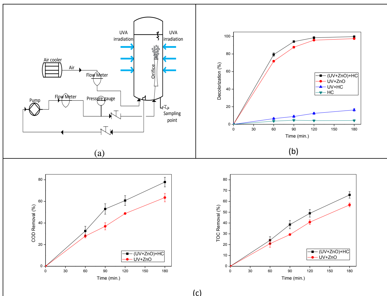
(a) Schematic design of the reactor (b) color removal and (c) mineralization of hybrid processes showing hydrodynamic cavitation and photocatalysis.
