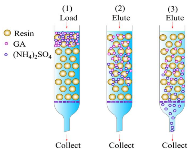
Fig.2. Schematic diagram of adsorption separation of GA.
