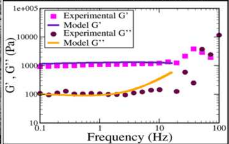
Storage, loss moduli for P. aeruginosa biofilm
