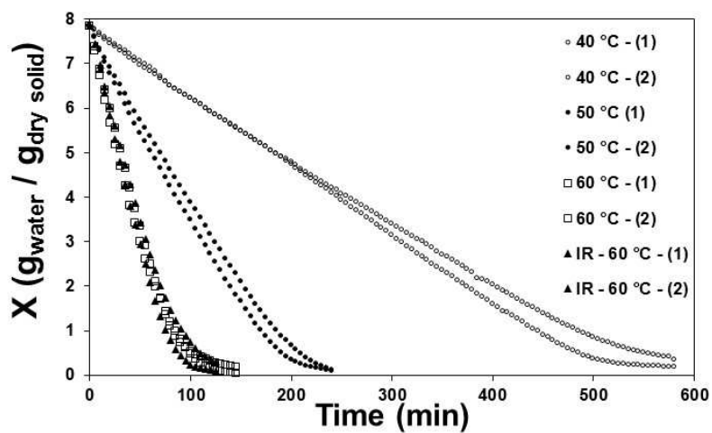
Drying conditions using tape casting
