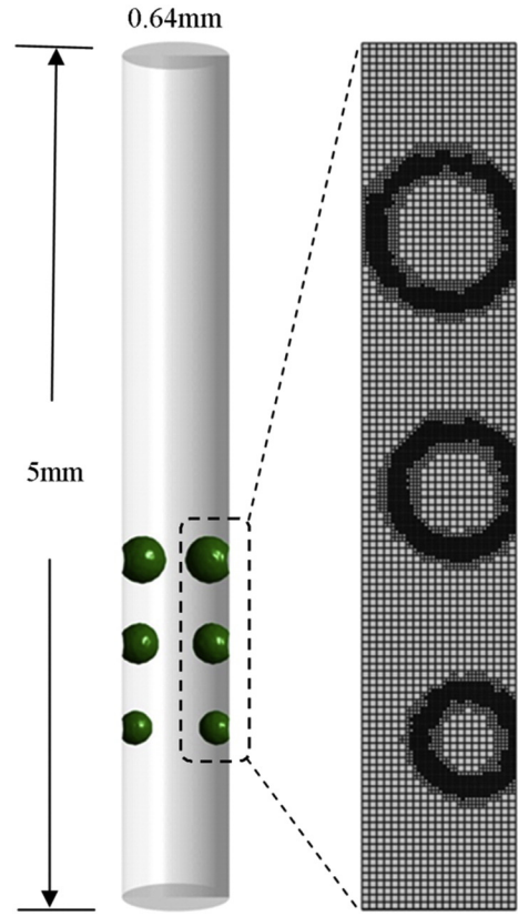
Fig. 1. The simulation domain is a 5 mm long cylindrical with a diameter of 0.64 mm. Bubbles' diameters are 0.1, 0.12 and 0.14 mm for cases with high saturated temperature (305.15 K) and 0.08, 0.1, and 0.12 mm for cases with low saturated temperature (300.15 K), respectively.
