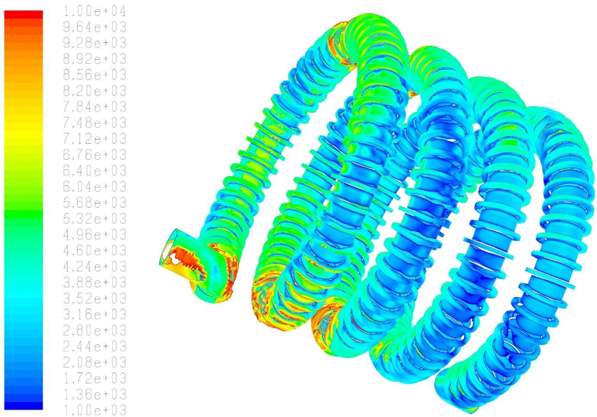
Contour of the local heat transfer rate coefficient (W/m 2 K)
