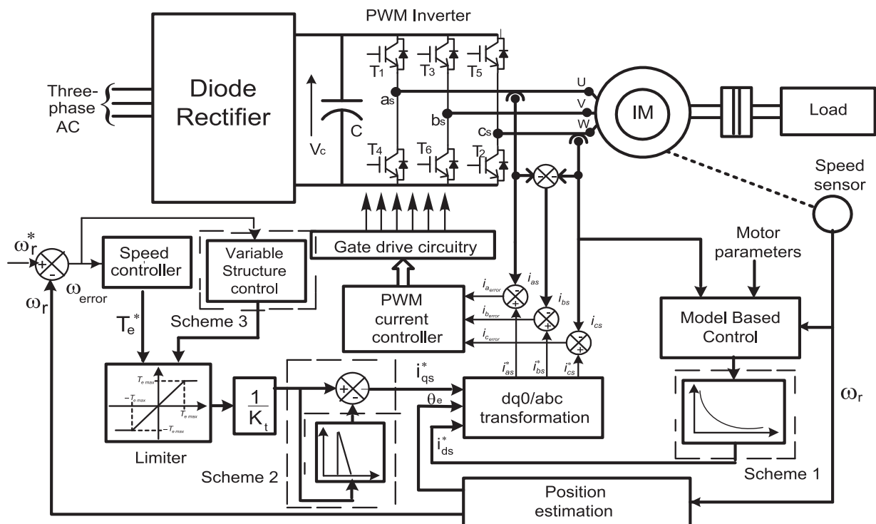
Fig. 1. MBC based vector controlled IM with proposed schemes.
