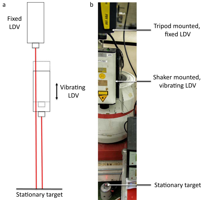
Fig. 1. Experimental arrangement showing vibrating and fixed LDVs to demonstrate sensitivity to instrument vibration; (a) schematic and (b) physical set-up.
