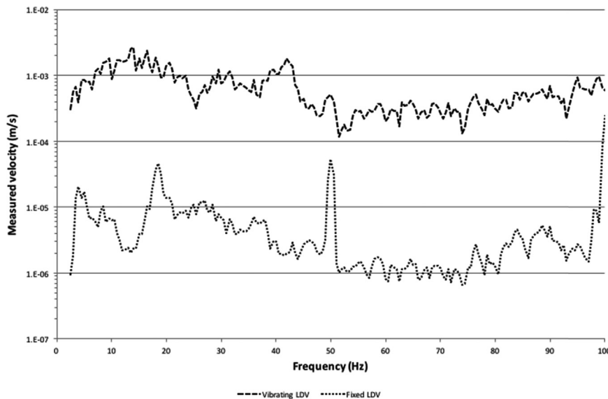
Fig. 2. Comparison between measurements from the vibrating LDV and from the fixed LDV on a (nominally) stationary target.
