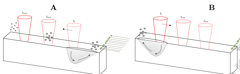
Figure 1: Schematic of laser beam scanning. A : scanning in the same direction as the flow. B : scanning against the direction of the flow, which might have caused more spattered powder.
