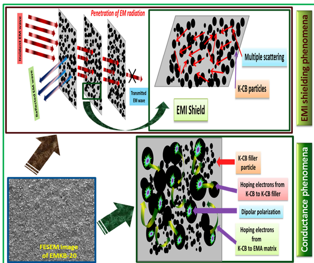
Graphical abstract: EMI shielding and conduction mechanism of the EMA/K-CB composites
