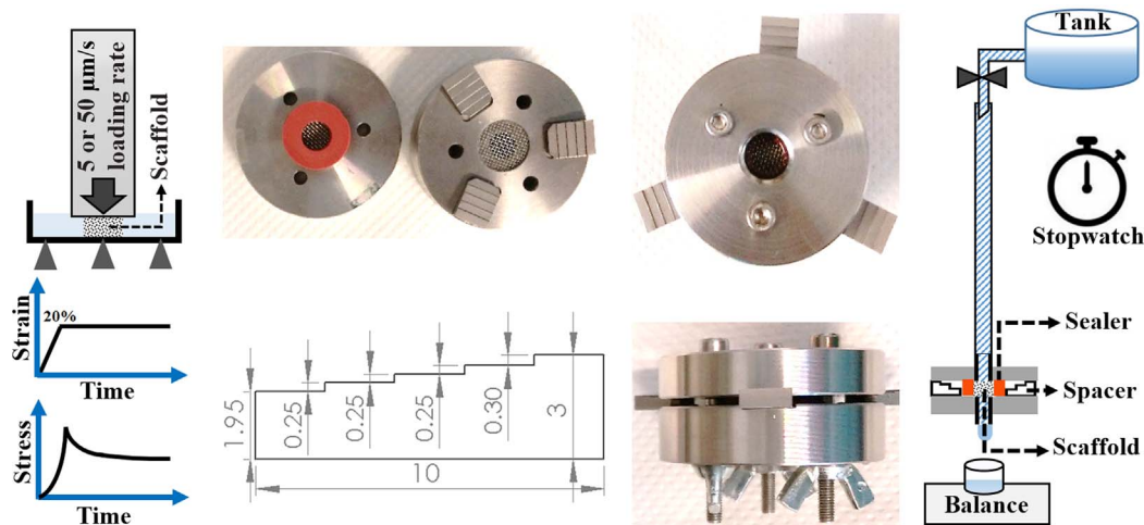
Fig. 1. Left: Schematic illustration of the stress relaxation test. Center: permeability chamber with stepwise spacer and the sealant. Right: schematics of the experimental setup to measure permeability of a scaffold under different compressive strains.
