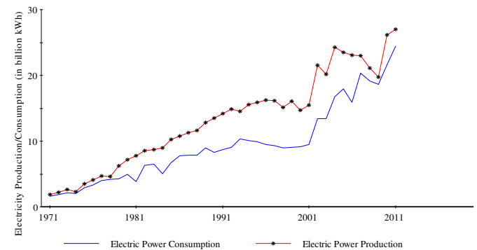
Fig. 1. Electricity production and consumption in Nigeria (1971–2011). Source: Constructed from the World Development Indicators (2014).
